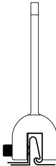
ASG4025-AL Milled Vertical Nail Flange 33/64" or Less Seam Width
