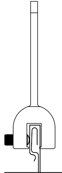
ASG4025-AL Snap Lock 13/32" or Less Seam Width
