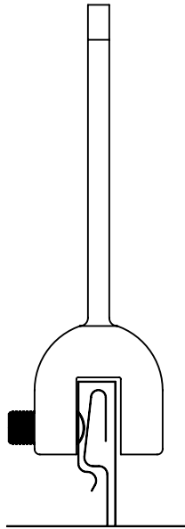
ASG4025-AL Milled Snap Lock 7/16"-33/64" Seam Width
