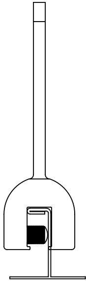
ASG4025-AL Single Lock 1/2" or Less Seam Width
