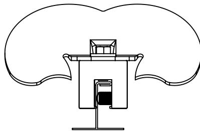
ASG33G-U-AL Single Lock 1/2" or Less Seam Width
